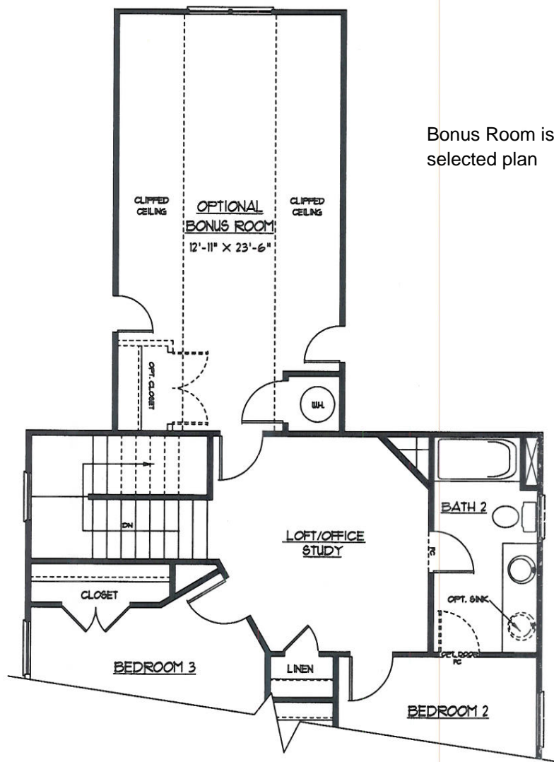
ALT. SECOND FLOOR COTSWOLD - B
