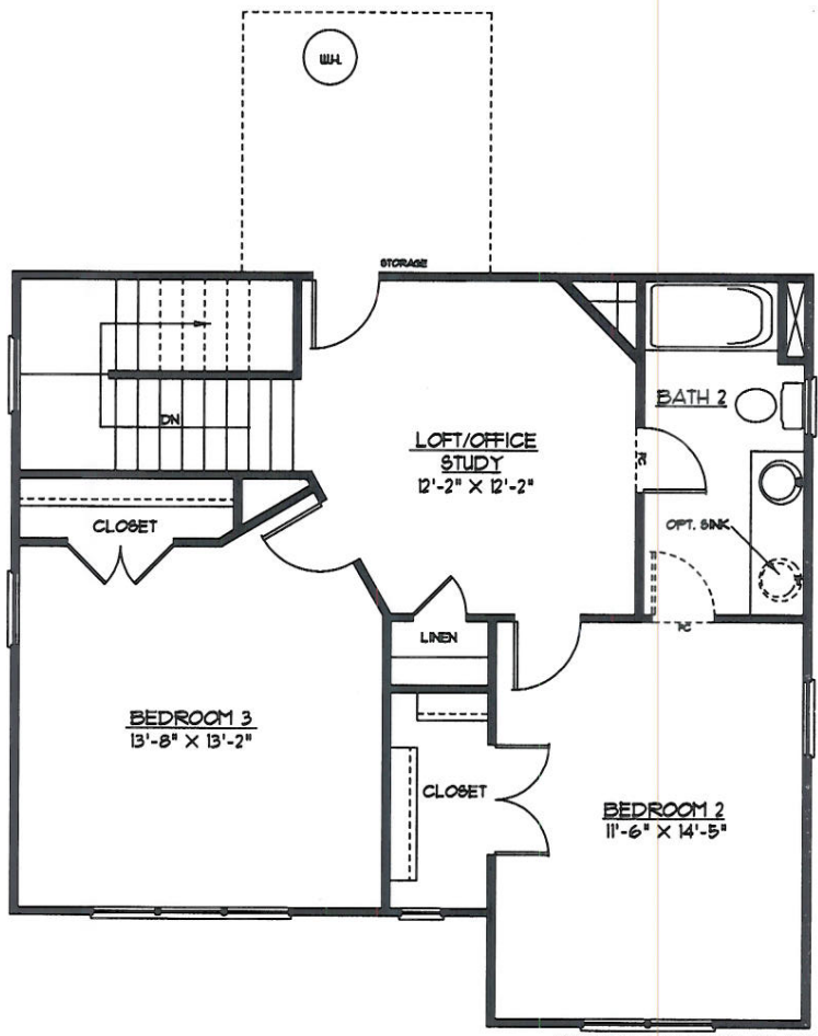
SECOND FLOOR PLAN COTSWOLD - B
